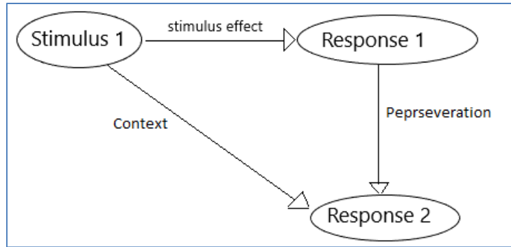
Figure 4. Correlation Analysis
